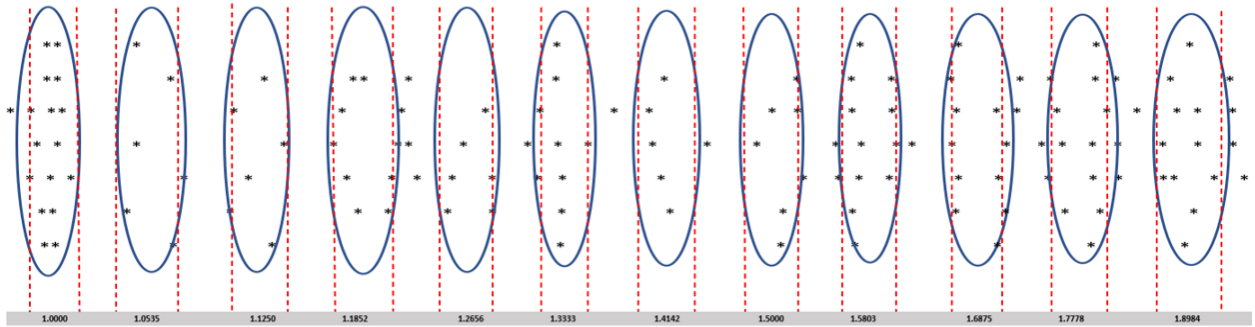
Distribution of Gravitational waves
