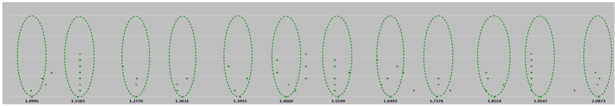
Spectral energy gaps of Hall effects
