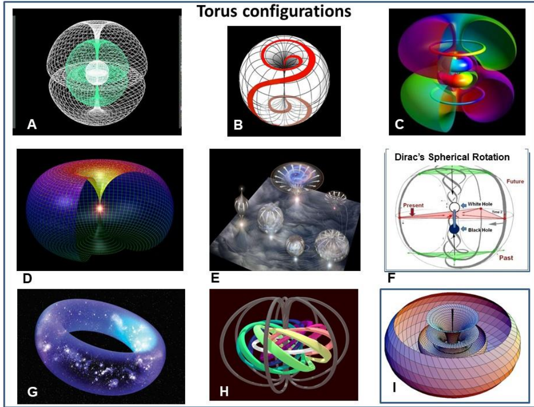
Figure 5. Various modalities of toroidal geometry: A: Nested torus structure B: Torus trajectory (red) C: Atomic structure as double torus, D: Filled space-time structure with singularity, E: Torus network, F: Dirac spherical rotation showing toroidal trajectories in relation to time G: Donut model of the universe, H: Knot structure in torus as metaphor for attractor/standing wave, I: cartoon of a twistor as a supposed space-time unit.
